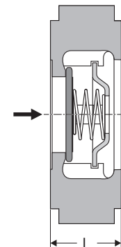
DN 125-200 mm (5–8") Standard design fitted with M8 antistatic connection
