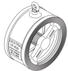
DN 125-200 mm (5–8") Standard design fitted with M8 antistatic connection
